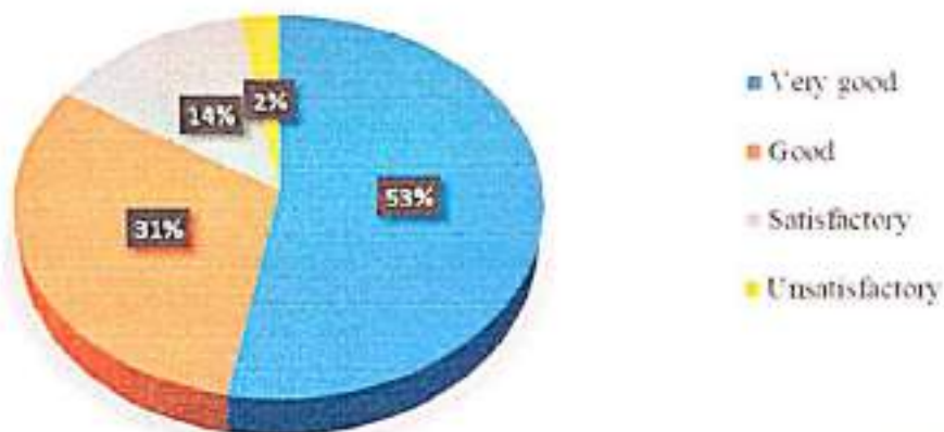
Student Feedback B.A. Programme (Percentage Score)
